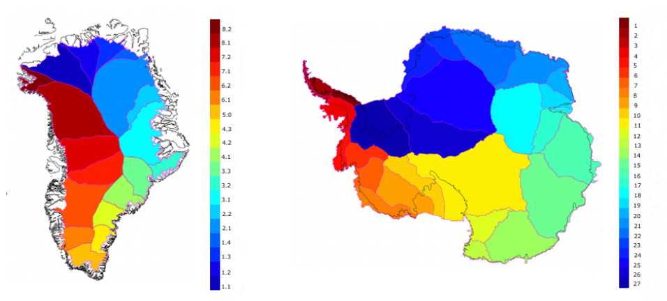
Figure 18. Cryo-TEMPO glaciological catchment masks, based upon the Zwally et al. (2012) definition. The 19 basins in Greenland are grouped into eight separate regions (1=North, 2=North-East, 3=East, 4=South-East, 5=South, 6=South-West, 7=West, 8=North-West).
