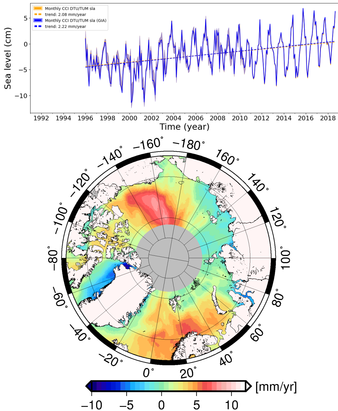
Figure 9. Top: Sea level trends and monthly averaged sea level anomalies of the Pan-Arctic. Bottom: Spatial sea level trends (Rose et.al. 2019)
