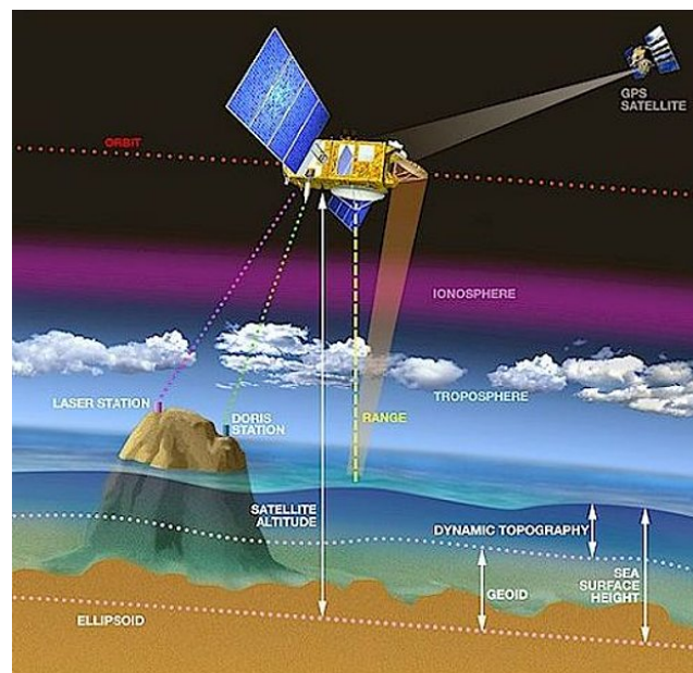
Figure 1. Example of altimetry principle over the ocean surface. The same principle is also valid over the others geophysical surfaces (e.g. ice and inland water surfaces). Image credit:
