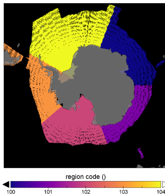
Figure 20. Example of sea ice regions codes for all SAR and SARin data the Southern Ocean.
