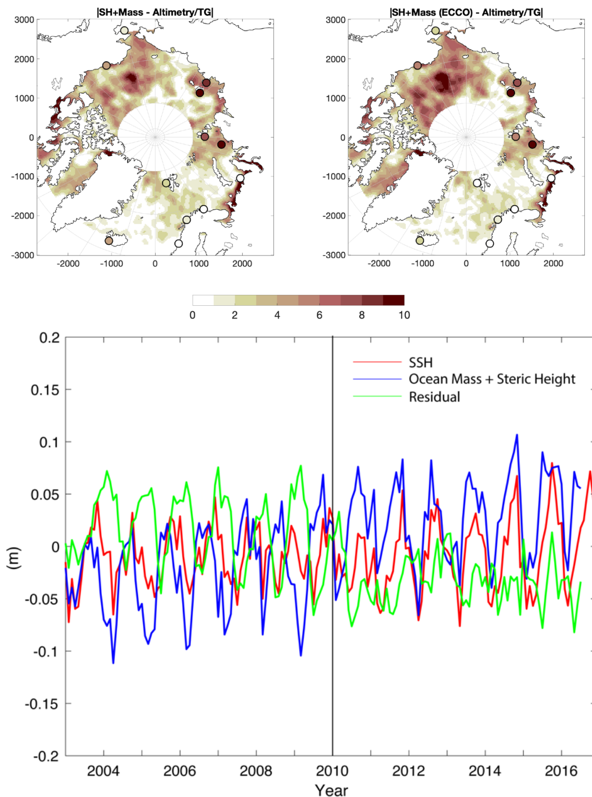
Figure 12. Sea level budget. Top: Spatial variability (from Ludwigsen et al., 2021). Bottom: temporal variability (from Raj et al., 2020).
