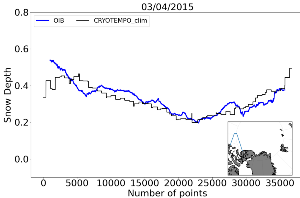
Figure 17: Snow depth along one OIB track in April 2015 for OIB in blue and the Cryo-TEMPO climatology in black.
