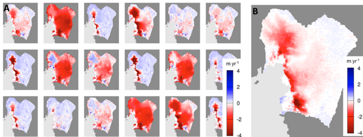
Figure 6. Rates of surface elevation change in the Amundsen Sea Sector of West Antarctica for a subset of a 284-member ensemble of BISICLE model simulations (A, adapted from Nias et al., 2016) and the Cryo-TEMPO TDP 2011-2021 mean (B).
