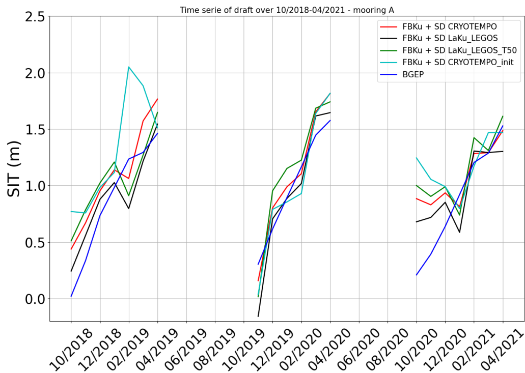
Figure 18: Time series of the sea ice thickness at a BGEP (Beaufort Gyre Exploration Project) mooring using BGEP data in blue and different snow depth products combined to the same Ku freeboard.
