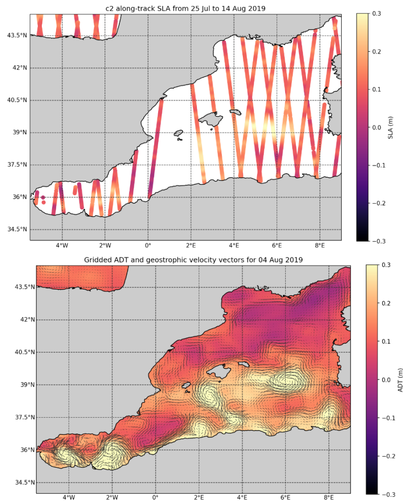
Figure 14. (Top) Example of observed along-track sea level anomaly (SLA) from CryoSat-2 from 25 July to 14 August 2019. (Bottom) Result of merging along-track observations from the multiple active altimeters (e.g. Jason-3, Sentinel-3, SARAL/ALtiKa etc.) to create daily level-4 maps of absolute dynamic topography (ADT; colour scale), which are in turn used to derive surface geostrophic velocities (vectors). More information on the generation and application of these products can be found in Taburet et al., 2019.
