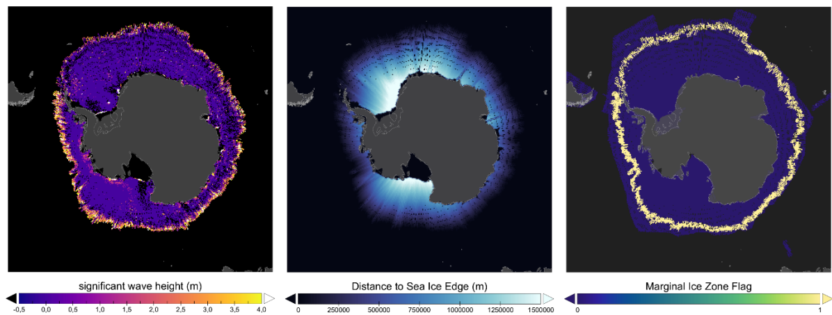
Figure 21: Significant wave height (left), distance to ice edge (center) and resulting marginal ice zone flag (right) for all orbits of September 2019 in the southern hemisphere.
