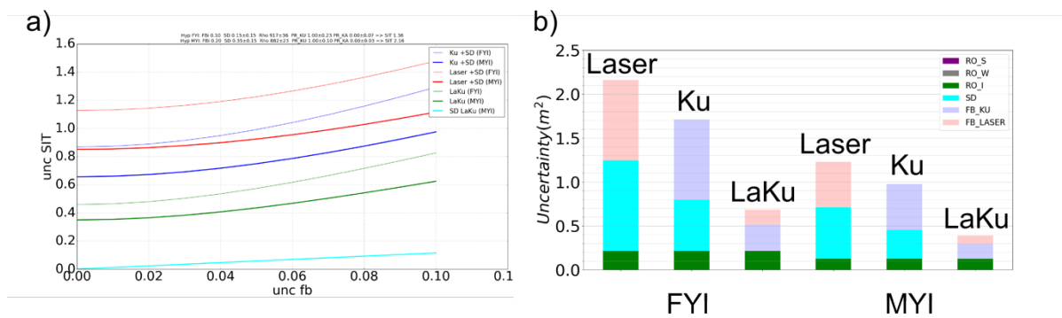
Figure 19: Left: Sea ice thickness uncertainties for a FYI (thin lines) and a MYI case (thick lines) as a function of the measured freeboard uncertainty using laser altimeter (in red), Ku altimeter (in dark blue), or combining Ku and Laser measurements (in green). For this last case we can also estimate the measured snow depth uncertainty (in light blue, the FYI and MYI curves are very close to each other, almost overlapping). The right part of this figure shows the relative contributions of each squared uncertainty on the SIT square uncertainty with freeboard of laser and Ku contributions in pink and light purple, snow depth in light blue, ice density in green, snow density in dark purple, water density in grey (too small to be visible).
